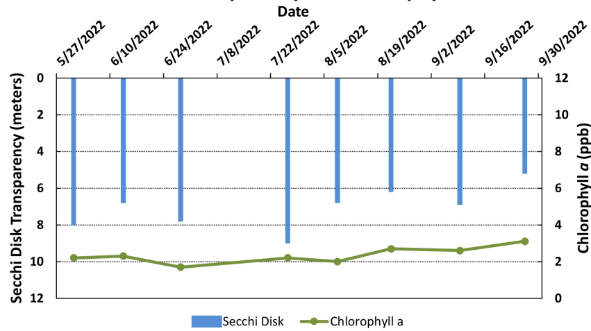
Figure 2. Lovell Lake (2022 Seasonal Data) Secchi Disk Transparency and Chlorophyll a Data
