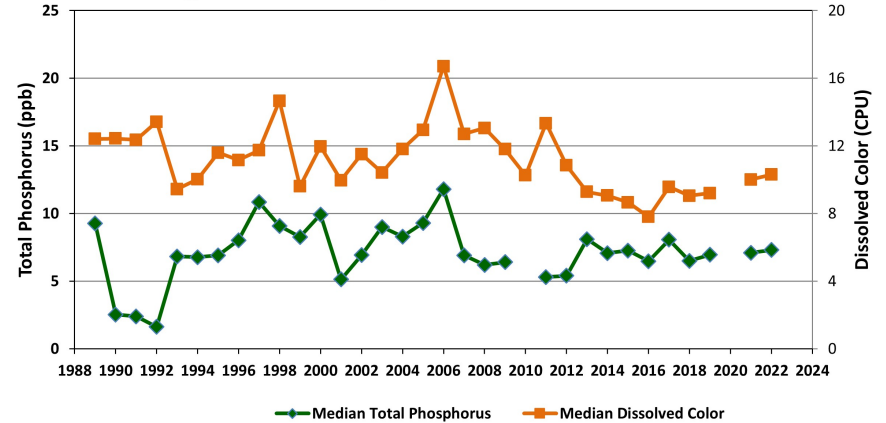
Figure 5. Lovell Lake - Site 2 South (1989-2022) Long-term Total Phosphorus and Dissolved Color Data
