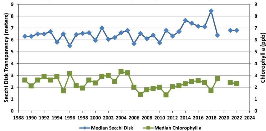
Figure 4. Lovell Lake - Site 2 South (1989-2022) Long-term Secchi Disk Transparency and Chlorophyll a Data
