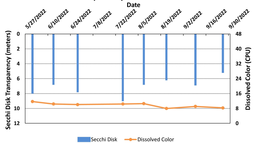
Figure 3. Lovell Lake (2022 Seasonal Data) Secchi Disk Transparency and Dissolved Color Data
