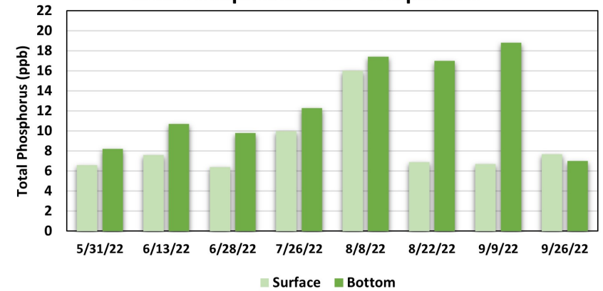
Figure 9. Lovell Lake - Site 2 South Total Phosphorus inter-comparison
