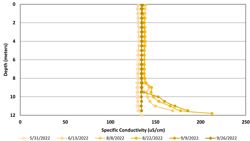
Figure 8. Lovell Lake - Site 2 South Specific Conductivity Profiles (May 31 through September 26, 2022)
