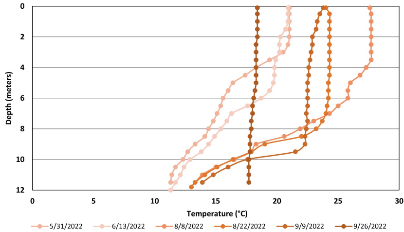
Figure 6. Lovell Lake - Site 2 South Temperature Profiles (May 31 through September 26, 2022)
