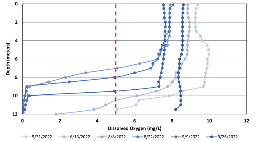
Figure 7. Lovell Lake - Site 2 South Dissolved Oxygen Profiles (May 31 through September 26, 2022)
