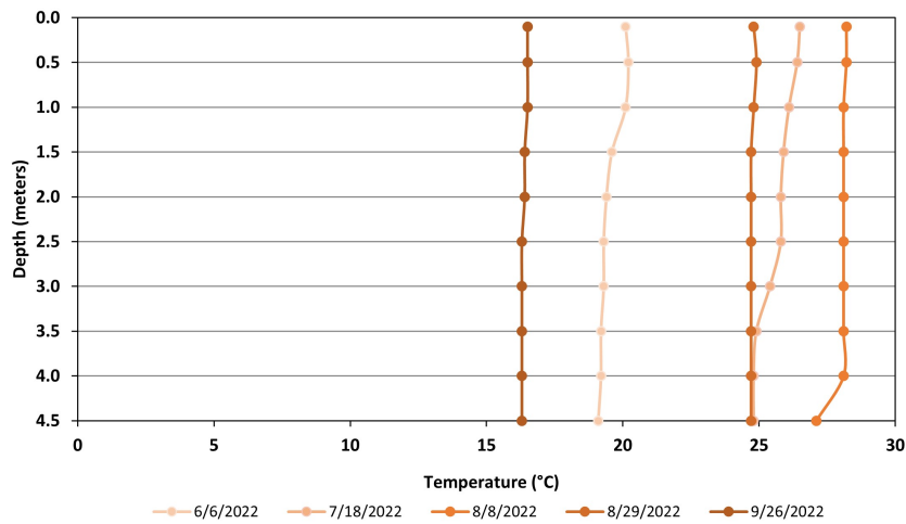
Figure 6. Province Lake - Site Deep Temperature Profiles (June 6 through September 26, 2022)
